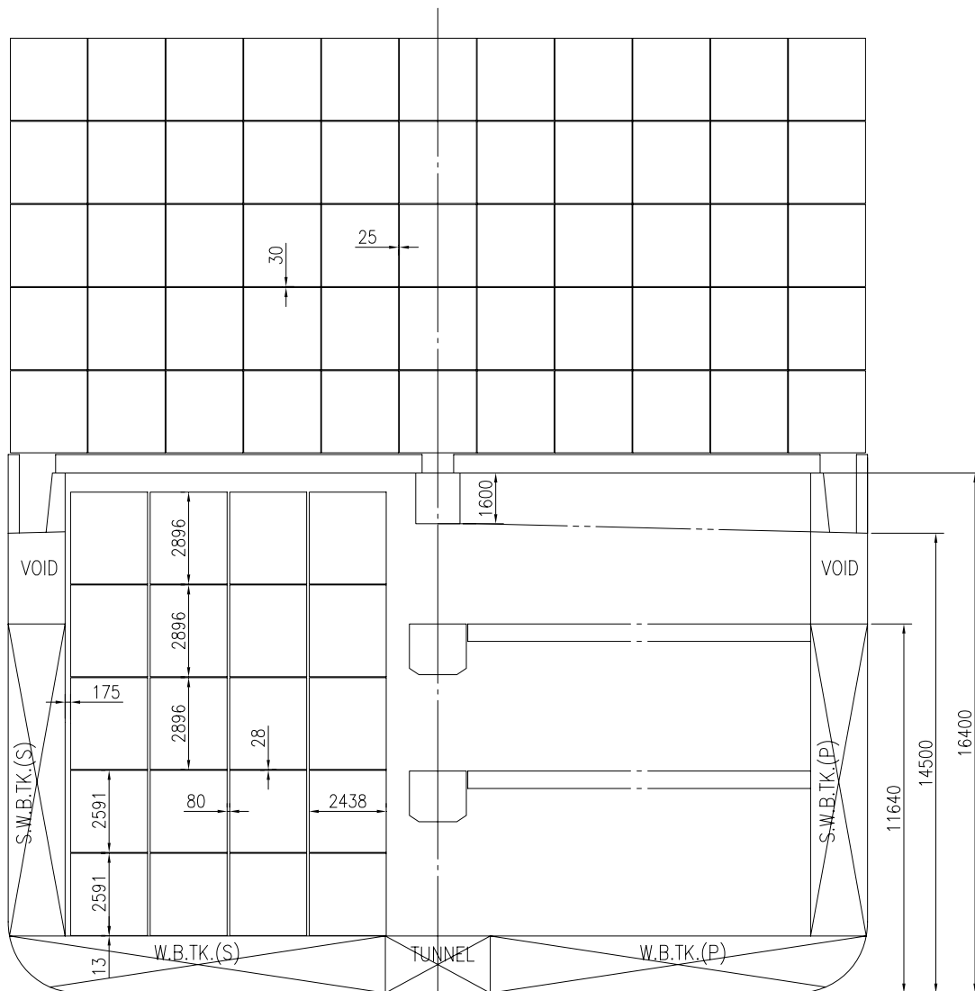
TYPICAL CARGO HOLD SECTION
