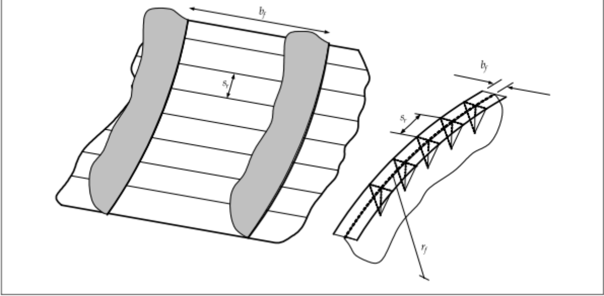
Figure 4.2.11 Curved Shell Panel and Face Plate
