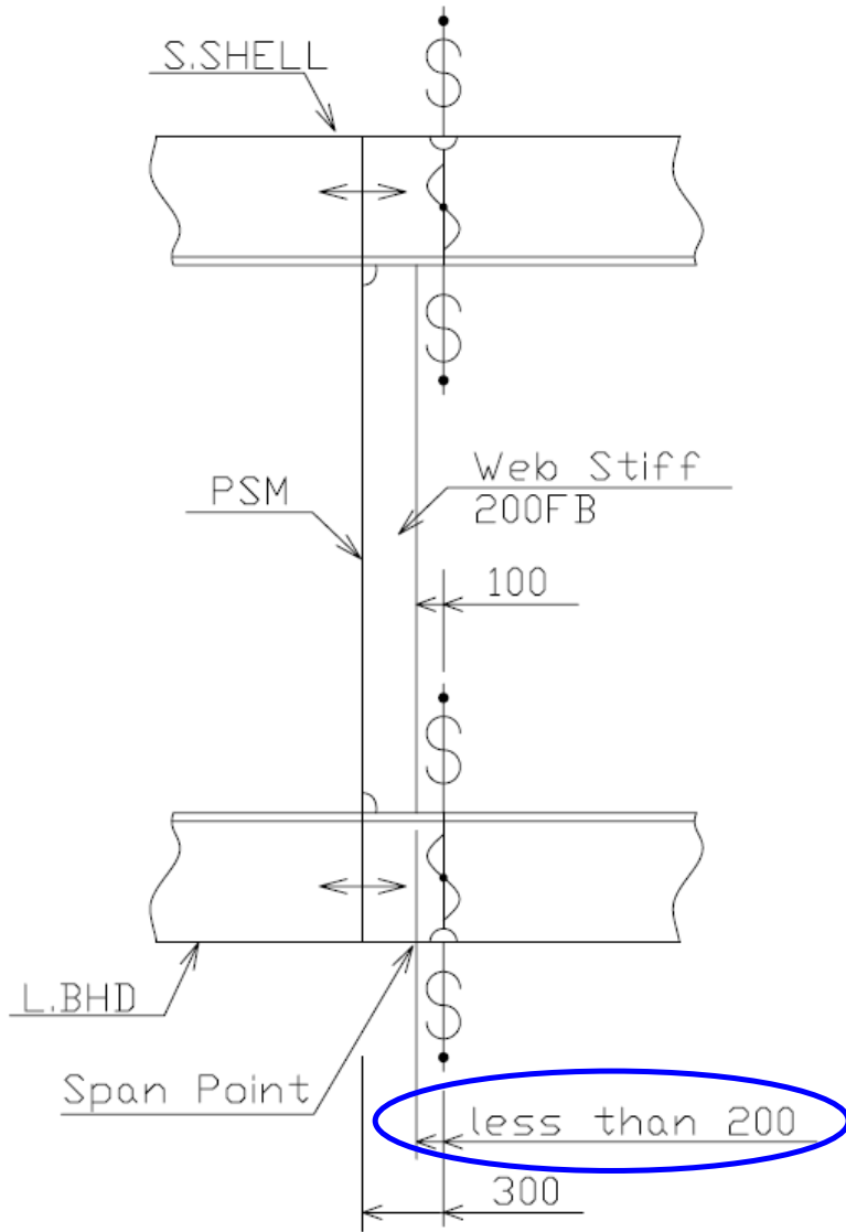
Fig.(c) Block butt arrangement in double skin construction(1)
