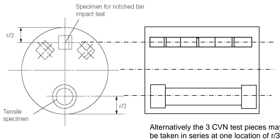
Figure 3 Sampling of steel bars, forgings and castings
