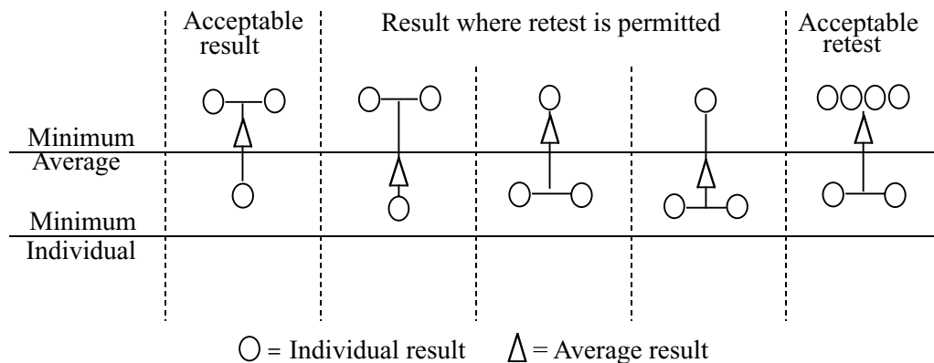
Figure 3 Diagram showing acceptance / rejection and retest criteria
