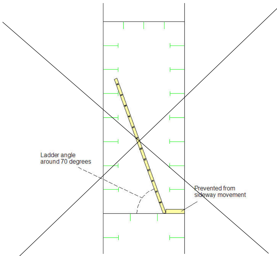
Fig.2 Use of Portable Ladder
