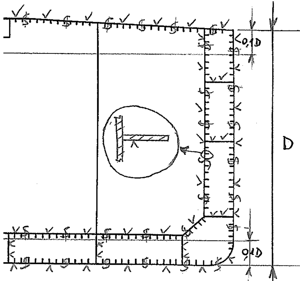
Figure 5 - Transverse section
