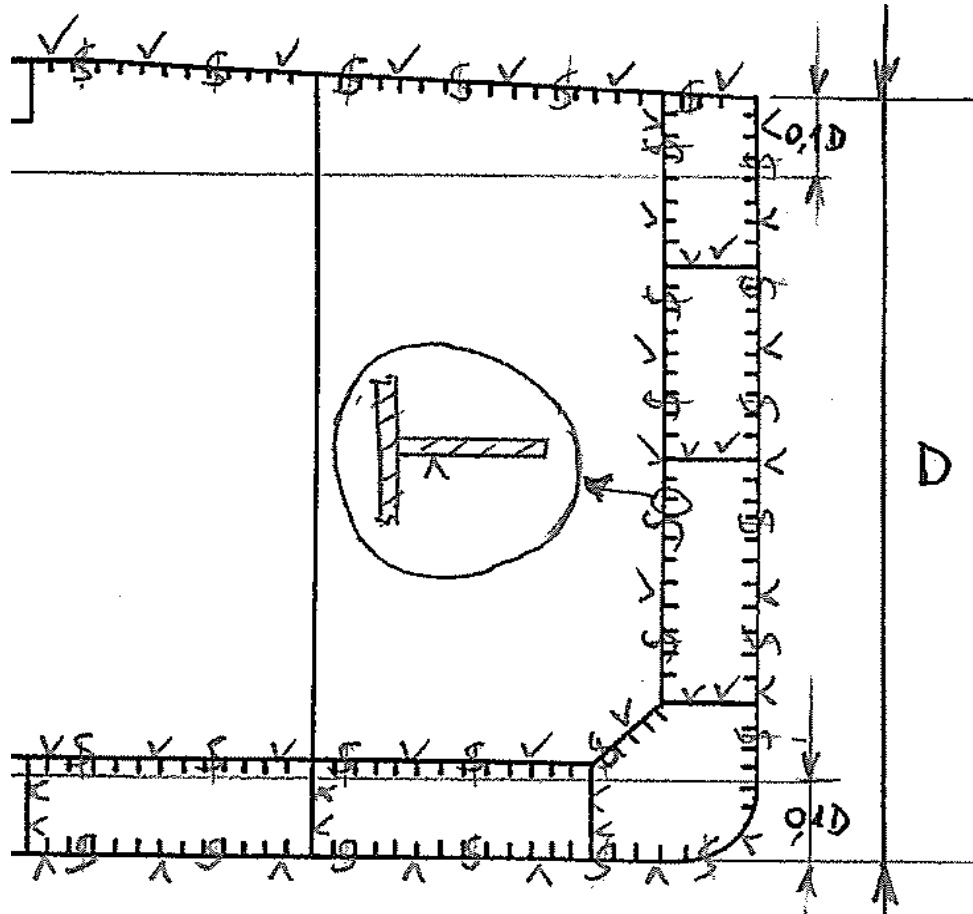
Figure 5 - Transverse section
