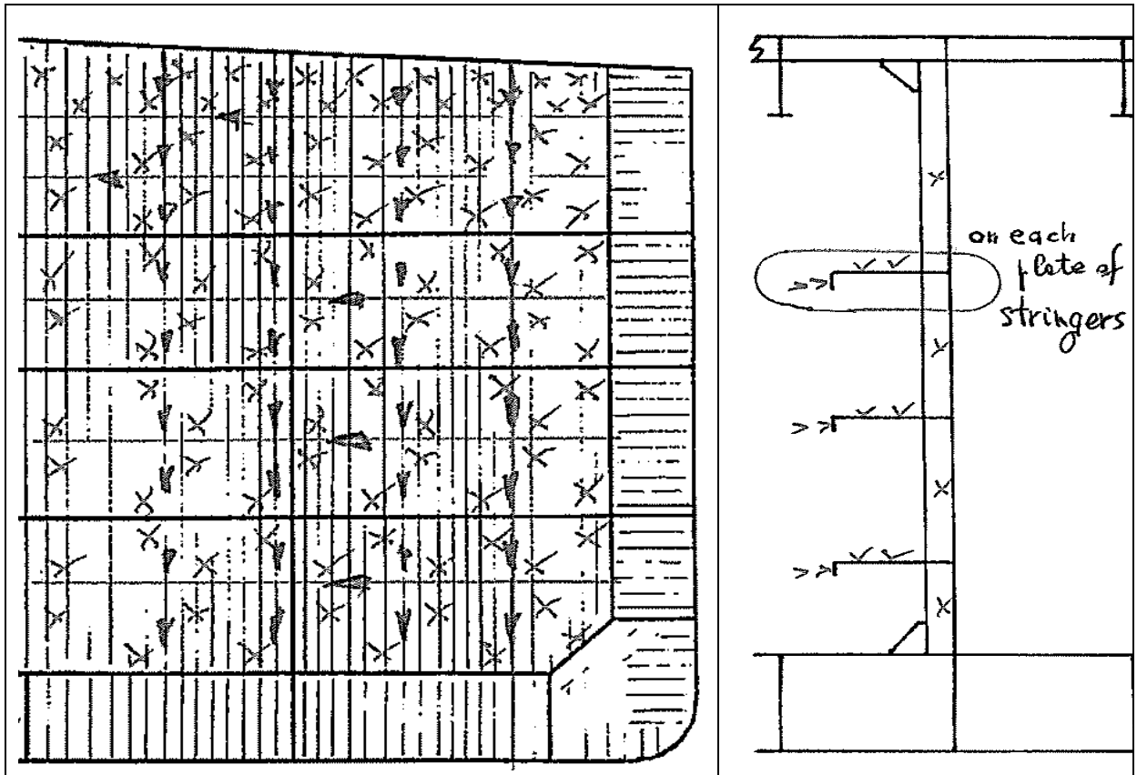
Figure 7 - Transverse bulkheads in cargo tanks
