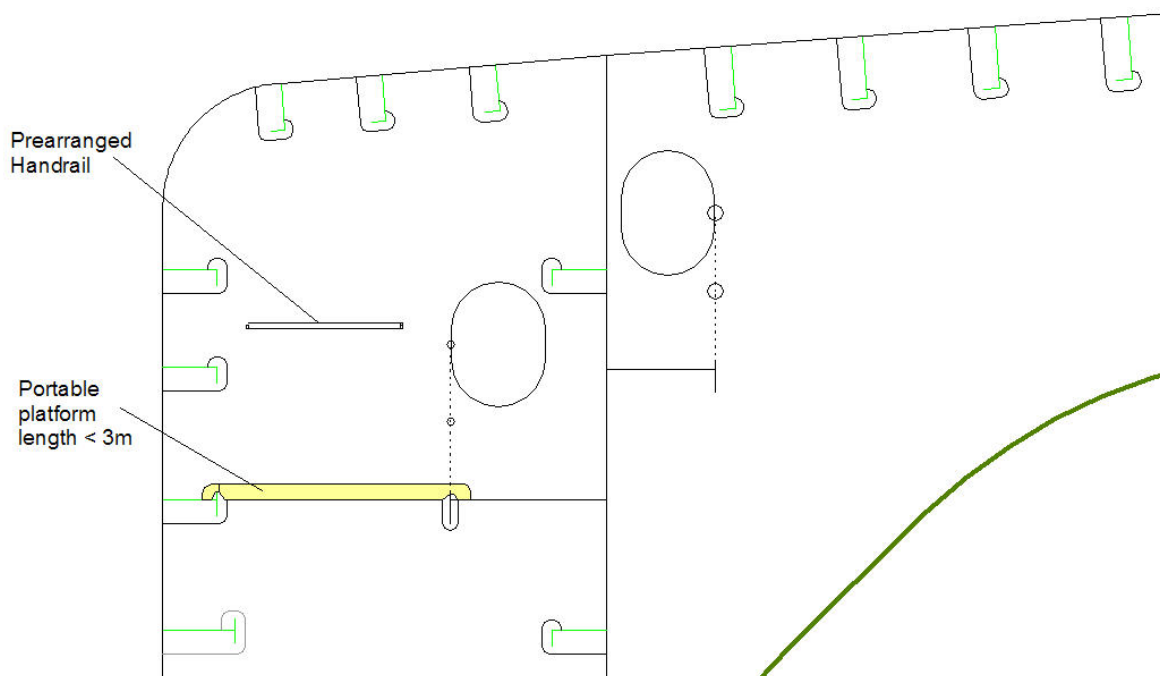
Fig.1 Portable Platform
